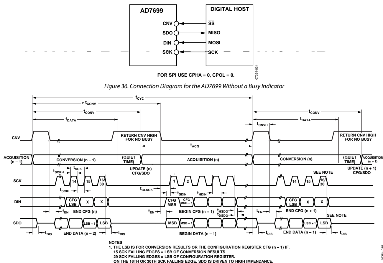
Figure 37. Serial Interface Timing for the AD7699 Without a Busy Indicator
