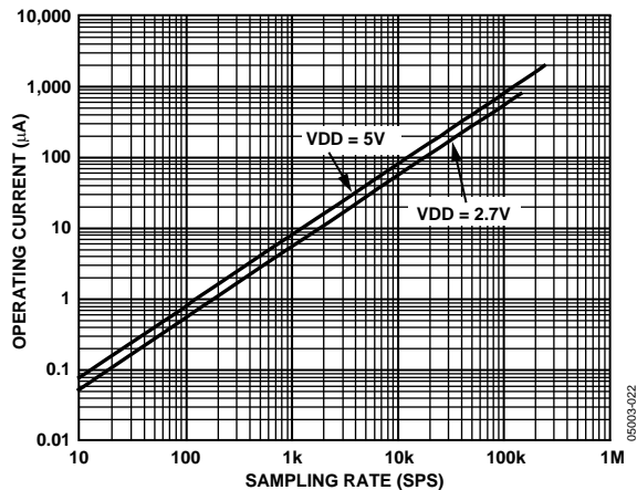
Figure 22. Operating Current vs. Sampling Rate
