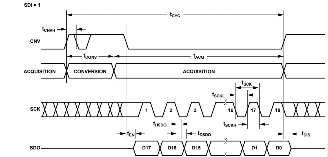
Figure 35. 3-Wire \overline{\text{CS}} Mode Without Busy Indicator Serial Interface Timing (SDI High)
