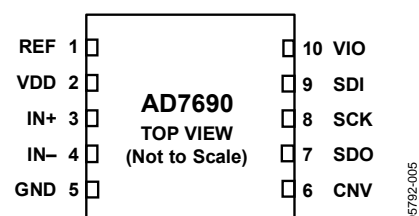
Figure 6. 10-Lead QFN (LFCSP) Pin Configuration
