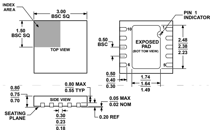
Figure 49. 10-Lead Lead Frame Chip Scale Package [QFN (LFCSP_WD)] 3 mm × 3 mm Body, Very Very Thin, Dual Lead (CP-10-9)
