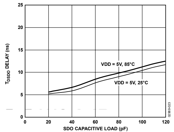
Figure 23. t_{\text{SDO}} Delay vs. Capacitance Load and Supply
