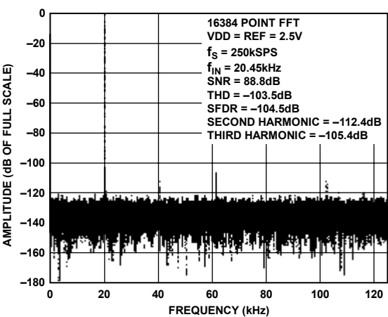
Figure 12. FFT Plot
