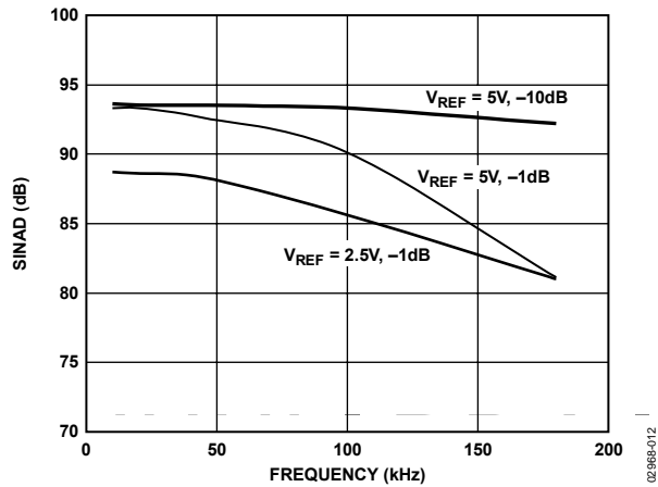
Figure 14. SINAD vs. Frequency
