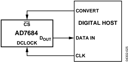
Figure 25. Connection Diagram
