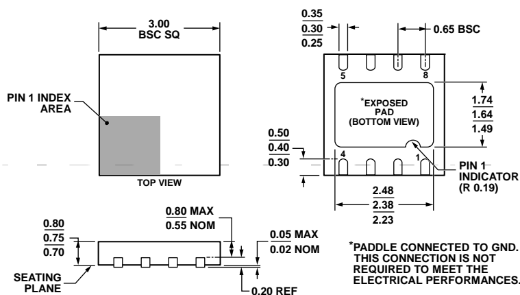
Figure 27. 8-Terminal Quad Flat No Lead Package (QFN) [LFCSP_WD] 3 mm × 3 mm Body, Very Very Thin, Dual Lead (CP-8-3) Dimensions Shown in millimeters
