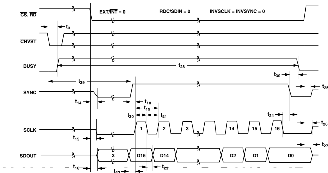
Figure 17. Master Serial Data Timing for Reading (Read after Convert)
