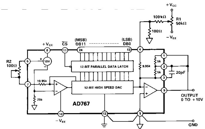
Figure 2. 0 to +10 \text{ V} Unipolar Voltage Output
