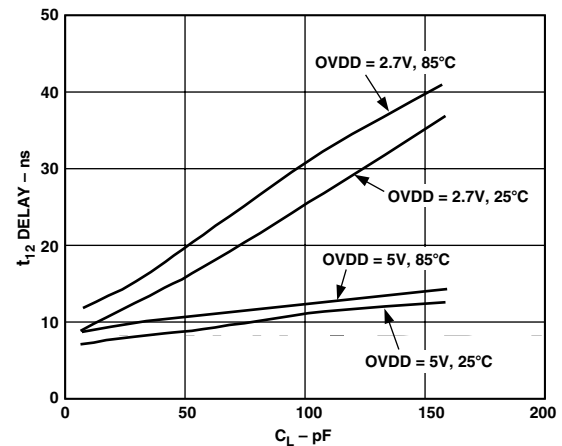
TPC 14. Typical Delay vs. Load Capacitance C L
