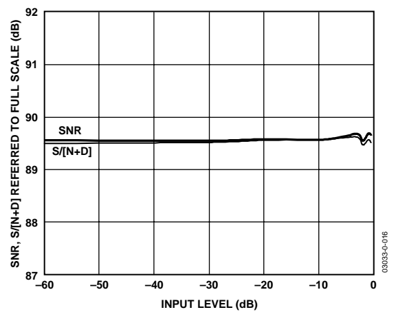
Figure 16. SNR and \text{S}/[\text{N}+\text{D}] vs. Input Level (Referred to Full Scale)
