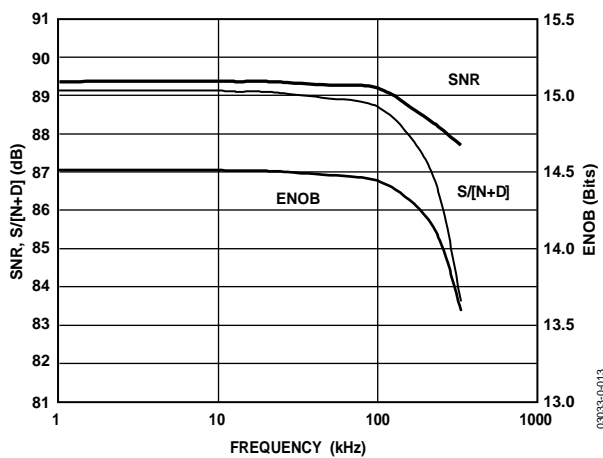
Figure 13. SNR, \text{S}/[\text{N}+\text{D}] , and ENOB vs. Frequency
