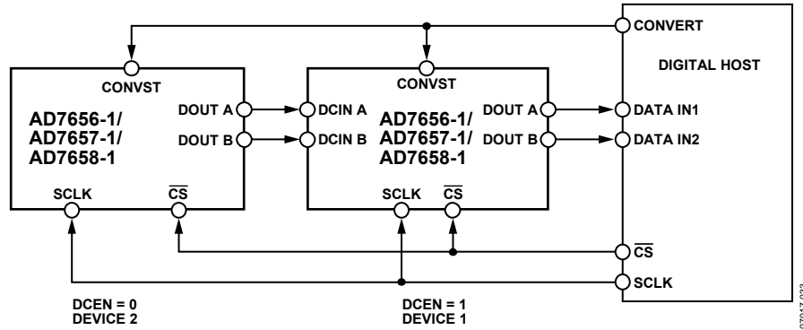
Figure 34. Daisy-Chain Configuration
