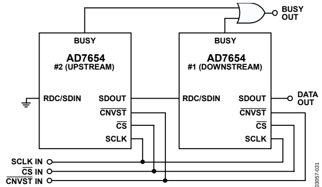
Figure 31. Two AD7654s in a Daisy-Chain Configuration
