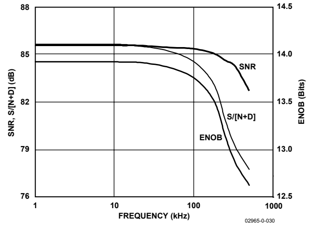
Figure 10. SNR, \text{S}/[\text{N}+\text{D}] , and ENOB vs. Frequency
