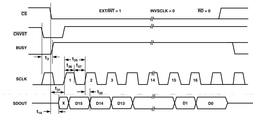
Figure 16. Slave Serial Data Timing for Reading (Read Previous Conversion During Convert)
