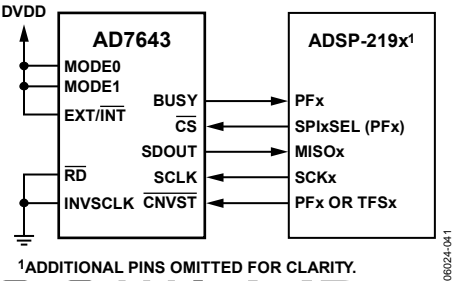
Figure 41. Interfacing the AD7643 to ADSP-219x
