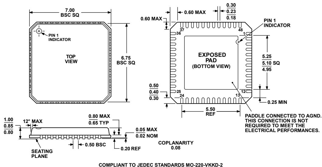
Figure 42. 48-Lead Lead Frame Chip Scale Package [LFCSP_VQ] 7 mm × 7 mm Body, Very Thin Quad (CP-48-1) Dimensions shown in millimeters
