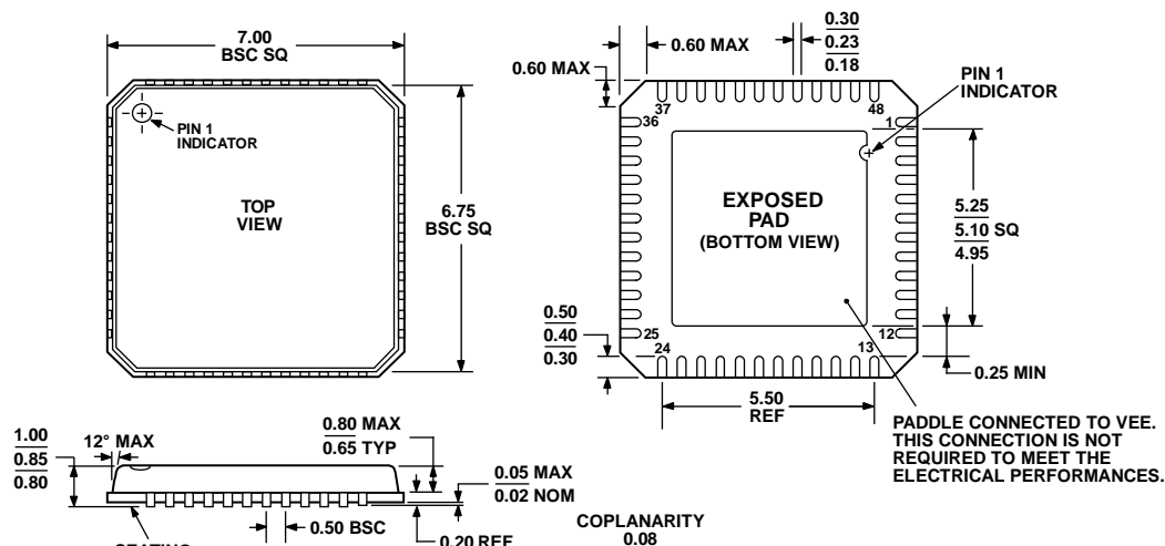
Figure 48. 48-Lead Lead Frame Chip Scale Package [LFCSP_VQ] 7 mm x 7 mm Body, Very Thin Quad (CP-48-1)
