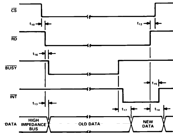
Figure 12. ADC Mode 2 Interface Timing
