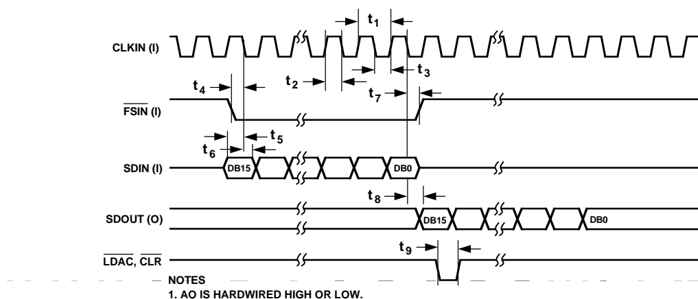
Figure 1. Timing Diagram
