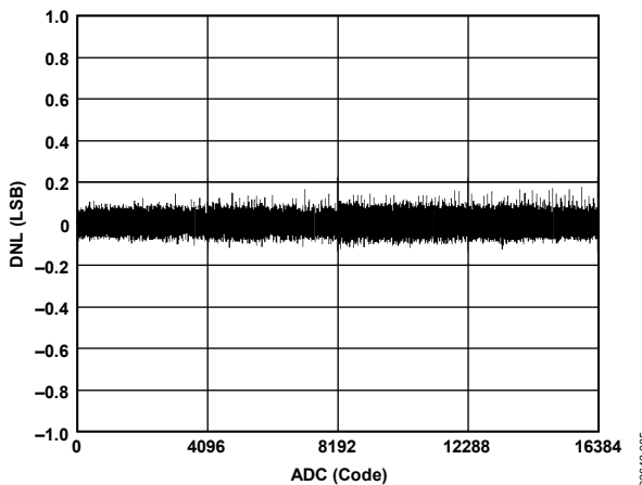
Figure 5. Typical DNL
