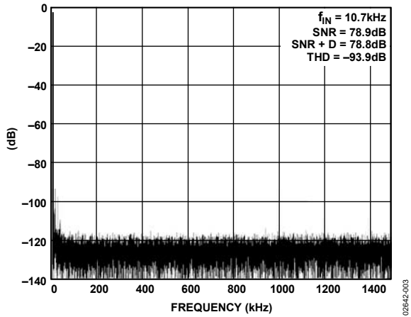
Figure 3. 64 k FFT Plot with 10 kHz Input Tone
