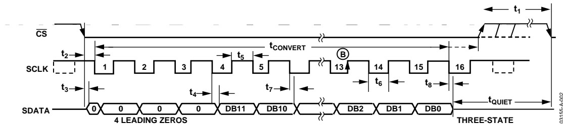
Figure 2. AD7453 Serial Interface Timing Diagram
