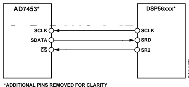
Figure 30. Interfacing to the DSP56xxx
