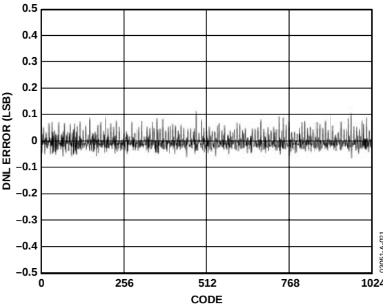
Figure 21. Typical DNL for the AD7440 for V_{DD} = 5\text{ V}
