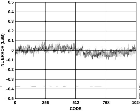
Figure 22. Typical INL for the AD7440 for V_{DD} = 5\text{ V}
