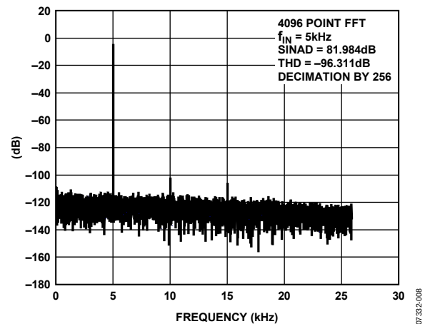
Figure 8. Typical FFT ( \pm 200\text{ mV} Range)
