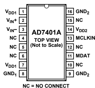
Figure 5. Pin Configuration
