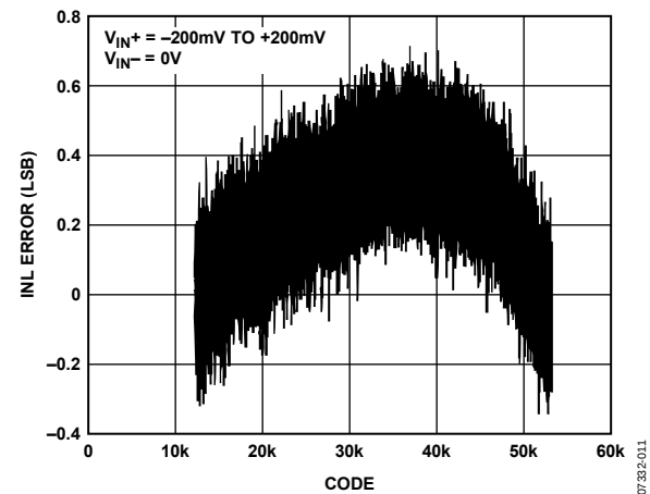
Figure 11. Typical INL ( \pm 200\text{ mV} Range)
