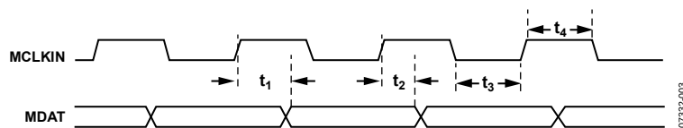
Figure 3. Data Timing
