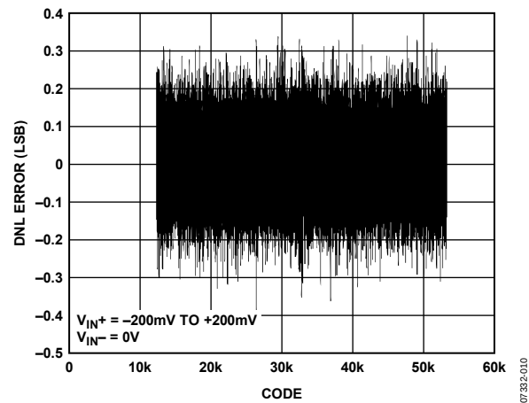
Figure 10. Typical DNL ( \pm 200\text{ mV} Range)
