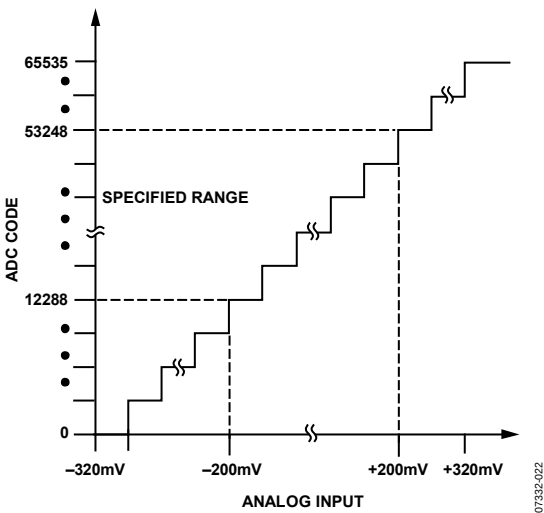
Figure 22. Filtered and Decimated 16-Bit Transfer Characteristic
