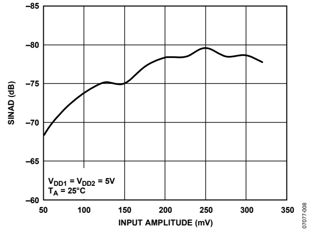
Figure 10. SINAD vs. V_{IN}
