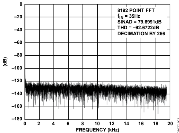
Figure 9. Typical FFT, \pm 200 mV Range (Using \text{Sinc}^3 Filter, 256 Decimation Rate)
