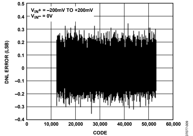
Figure 11. Typical DNL, \pm 200 mV Range (Using \text{Sinc}^3 Filter, 256 Decimation Rate)
