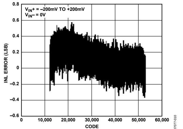
Figure 12. Typical INL, \pm 200 mV Range (Using \text{Sinc}^3 Filter, 256 Decimation Rate)
