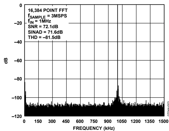
Figure 3. Typical FFT
