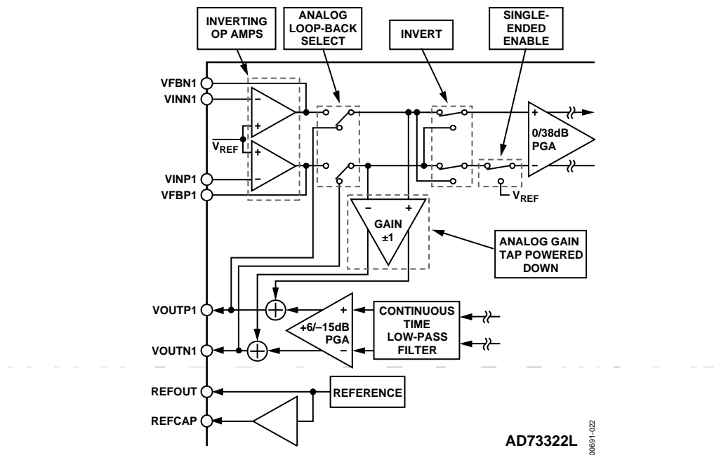
Figure 22. Analog Loop-Back Connectivity
