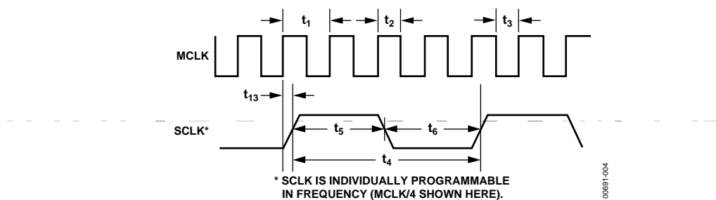
Figure 4. SCLK Timing
