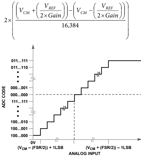
Figure 25. Twos Complement Transfer Function
