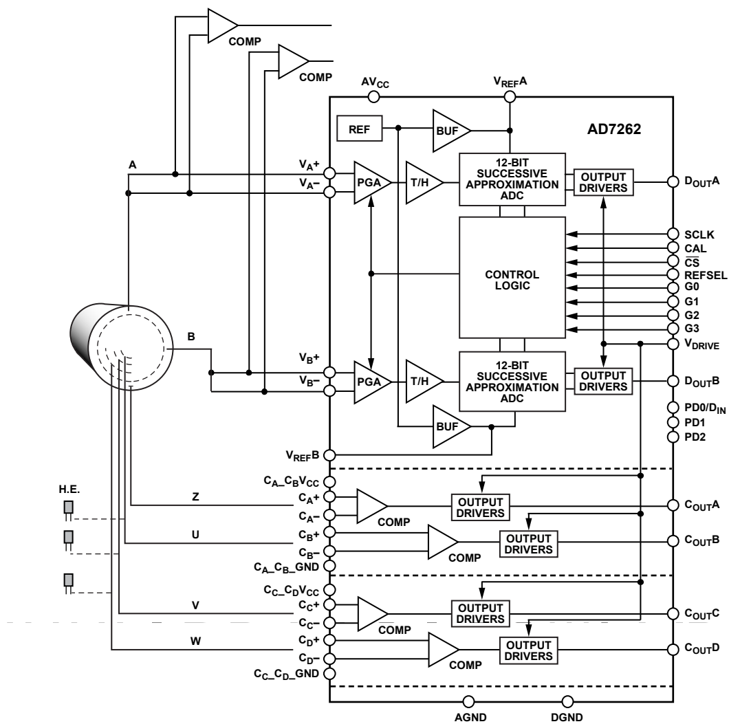
Figure 29. Typical System Connection Diagram with Optical Encoder
