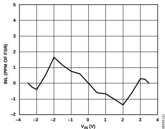
Figure 11. INL (Gain = 1)
