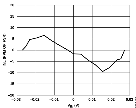
Figure 12. INL (Gain = 128)
