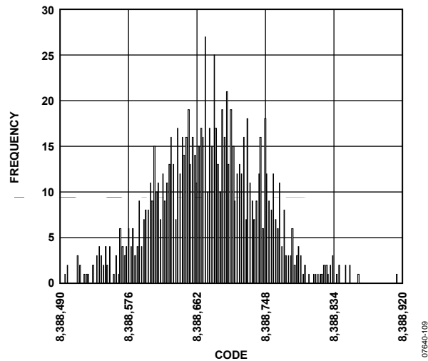
Figure 9. Noise Distribution Histogram ( V_{REF} = 5\text{ V} , Output Data Rate = 4800 Hz, Gain = 128, Chop Disabled, \text{Sinc}^4 Filter)
