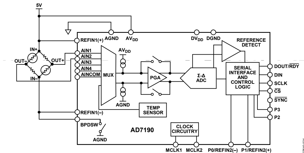
Figure 32. Typical Application (Weigh Scale)
