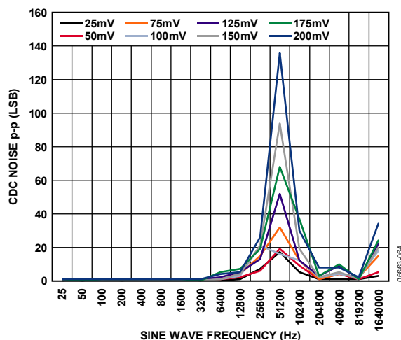
Figure 16. Power Supply Sine Wave Rejection, V_{CC} = 3.6\text{ V}
