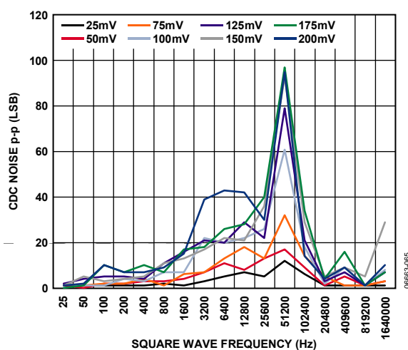
Figure 17. Power Supply Square Wave Rejection, V_{CC} = 3.6\text{ V}
