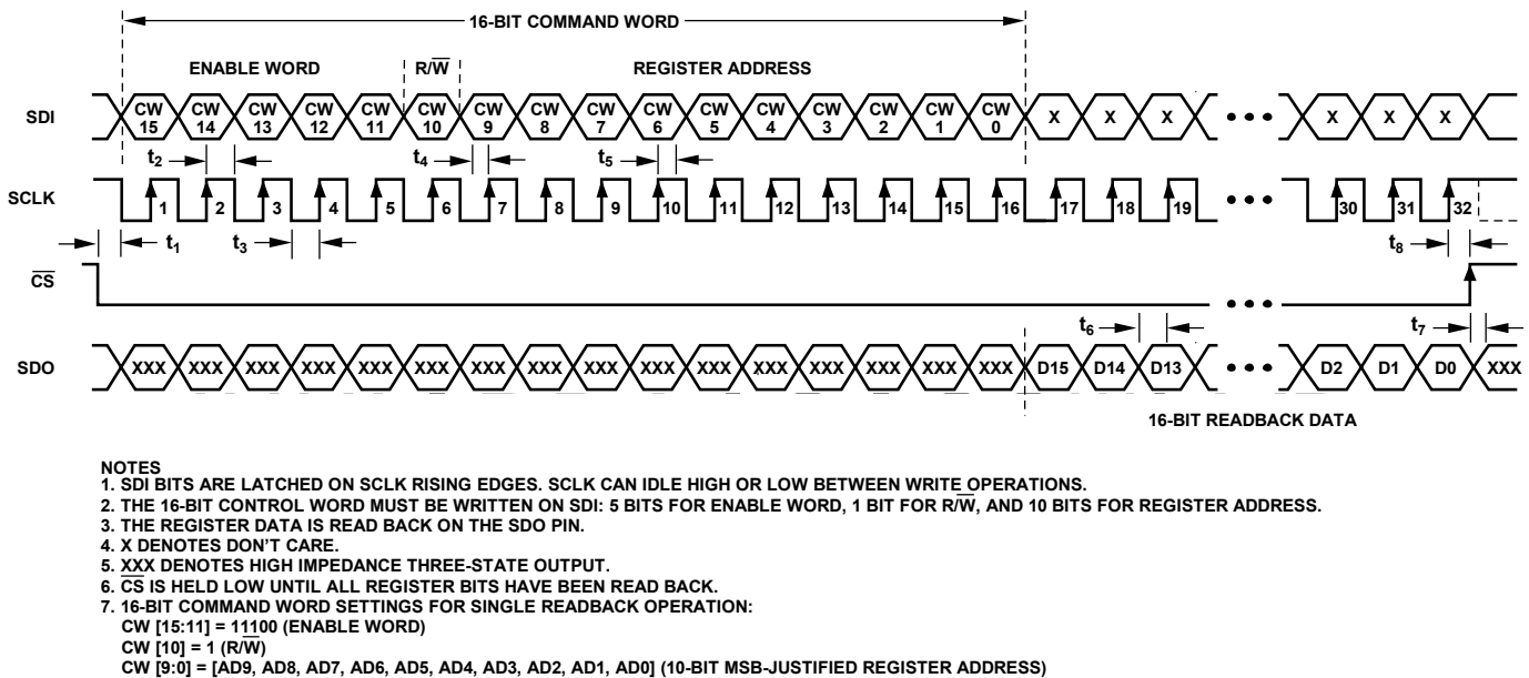
Figure 51. Single Register Readback SPI Timing
