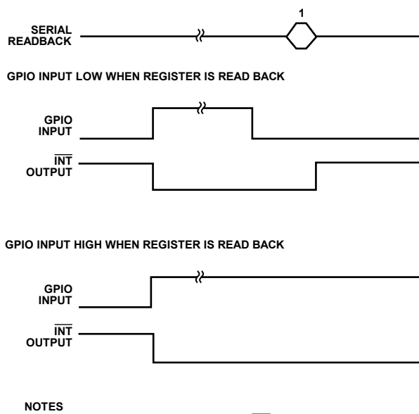
Figure 46. Example of \overline{\text{INT}} Output Controlled by the GPIO Input (GPIO_SETUP = 01, GPIO_INPUT_CONFIG = 11)
