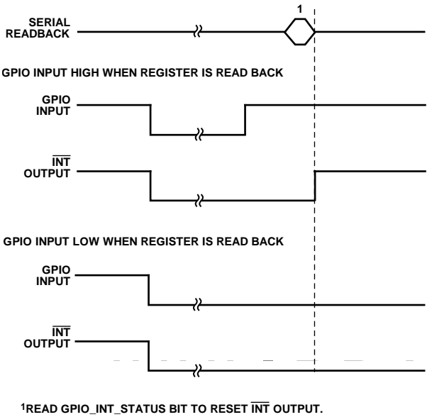
Figure 43. Example of \overline{\text{INT}} Output Controlled by the GPIO Input ( \text{GPIO\_SETUP} = 01 , \text{GPIO\_INPUT\_CONFIG} = 00 )
