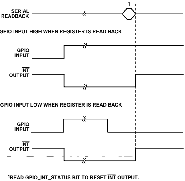
Figure 44. Example of \overline{\text{INT}} Output Controlled by the GPIO Input ( \text{GPIO\_SETUP} = 01 , \text{GPIO\_INPUT\_CONFIG} = 01 )
