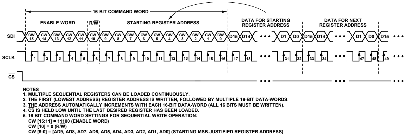
Figure 50. Sequential Register Write SPI Timing
