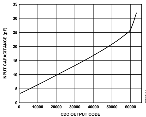
Figure 18. CDC Linearity, V_{CC} = 3.3\text{ V}
