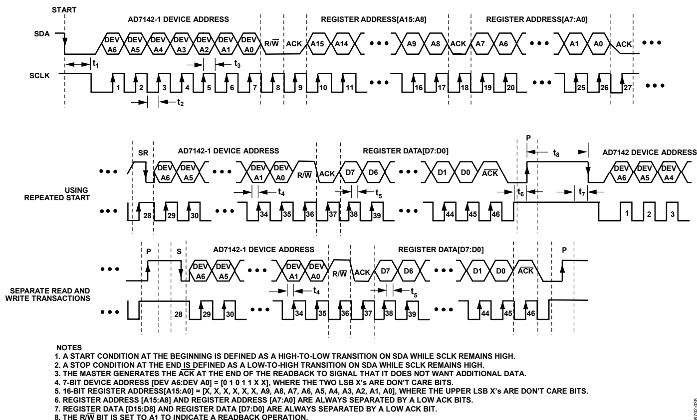
Figure 51. Example of I²C Timing for Single Register Readback Operation
