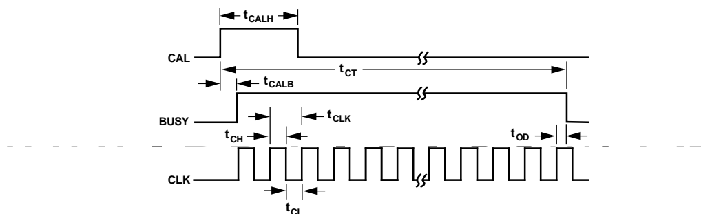
Figure 1. Calibration Timing
