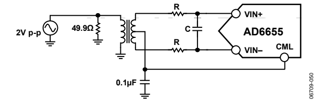
Figure 48. Differential Transformer-Coupled Configuration
