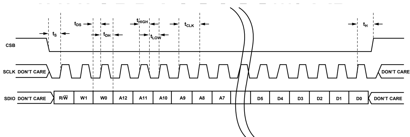
Figure 81. Serial Port Interface Timing Diagram
