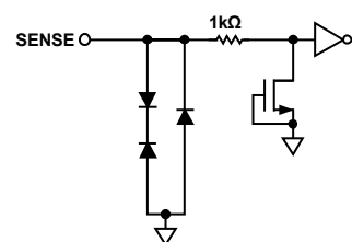
Figure 16. Equivalent SENSE Circuit
