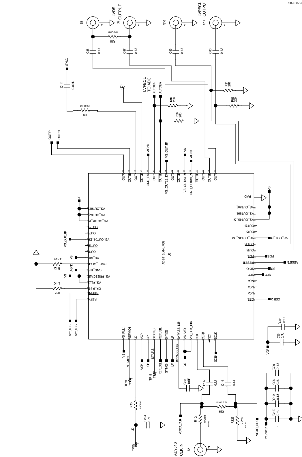
Figure 88. Evaluation Board Schematic, Optional AD9516 Clock Circuit
