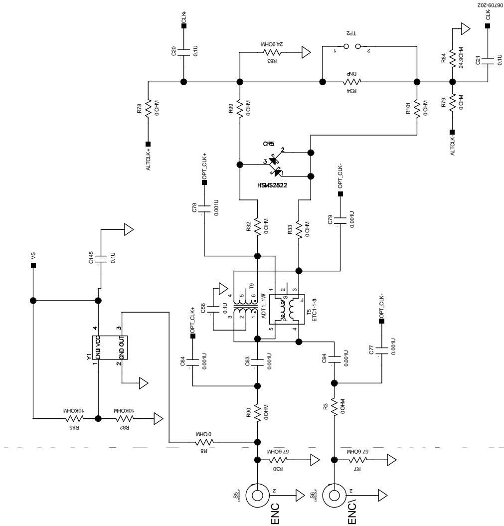
Figure 87. Evaluation Board Schematic, DUT Clock Input
