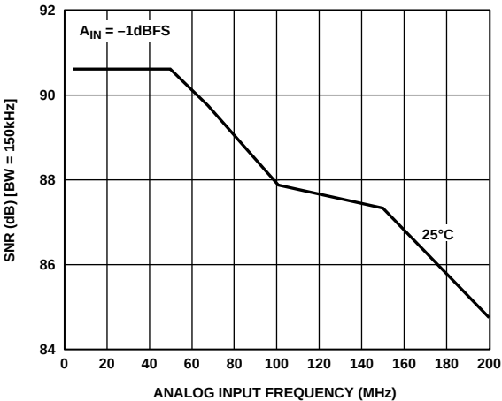
Figure 16. Noise vs. Analog Frequency (IF)
