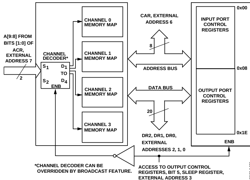
Figure 63. Block Diagram of the AD6652 Internal Memory Maps and Controls
