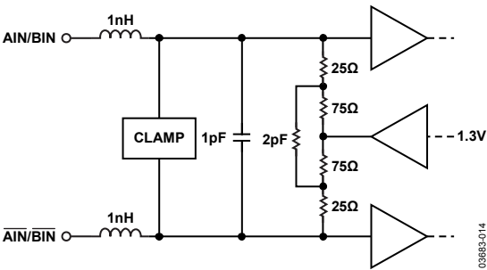
Figure 19. Analog Input
