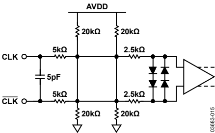
Figure 20. Clock Input
