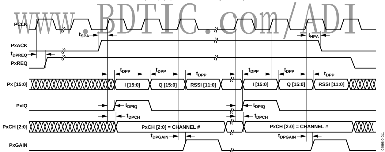
Figure 11. Master Mode PxACK to PCLK Switching Characteristics (x = A, B, C, D for Individual Output Ports)
