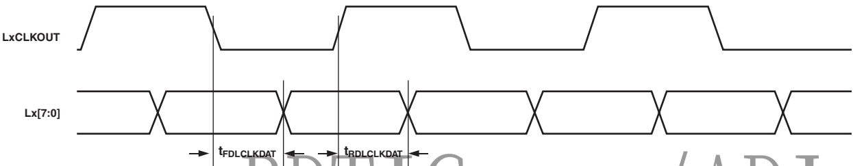
Figure 18. LxCLKOUT to Lx[7:0] Data Switching Characteristics
