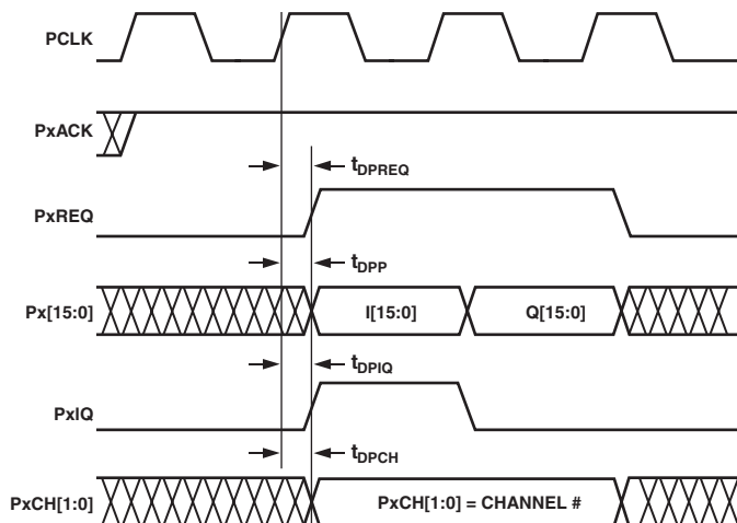
Figure 36. Channel Mode Interleaved Format
