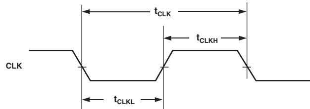
Figure 26. CLK Timing Requirements
