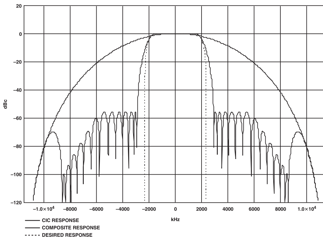
Figure 24. The Filter Above Is Designed to Meet UMTS Specifications. For this configuration, the clock is set to 76.8 MSPS with 20× chip rate (3.84 MCPS) and a 2× output data rate of 7.68 MCPS using two channels of the AD6634.
