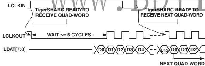
Figure 43. Link Port Data Transfer
