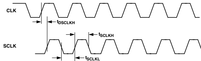
Figure 4. SCLK Switching Characteristics (Divide by 1)
