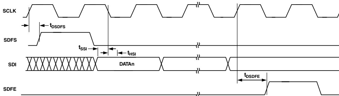
Figure 7. Serial Port Switching Characteristics
