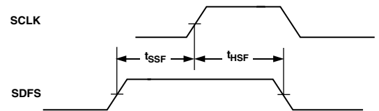
Figure 41. SDFS Timing Requirements (SBM = 0)
