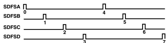
Figure 21. SDFS Timing for WBCDMA
