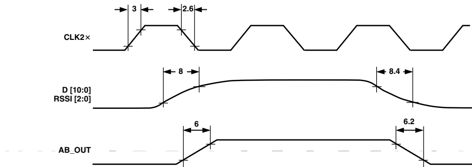
Figure 12. Typical Output Rise and Fall Times
