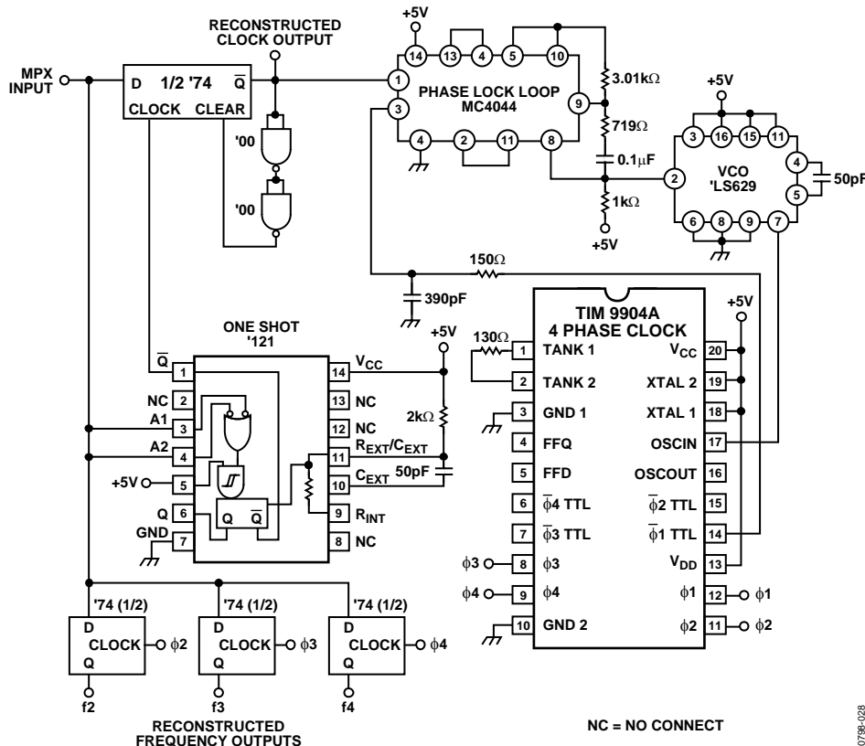
Figure 30. SVFC Demultiplexers
