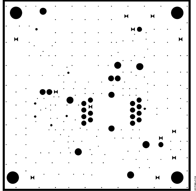
Figure 28. Evaluation Board—Internal Ground Plane
