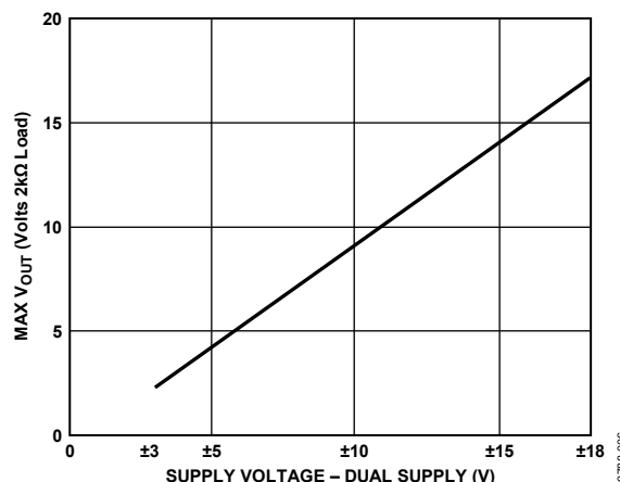
Figure 6. Maximum V_{OUT} vs. Supply Voltage
