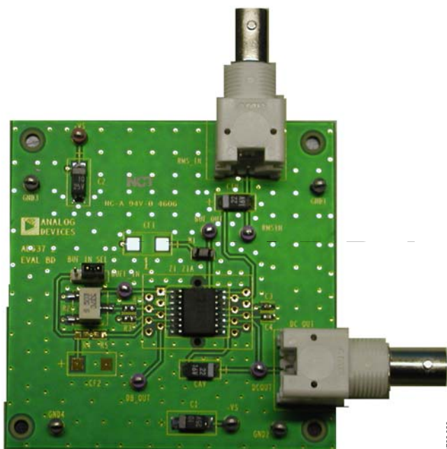
Figure 23. Evaluation Board
