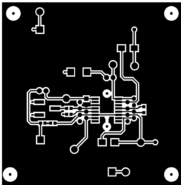
Figure 25. Evaluation Board—Component Side Copper
