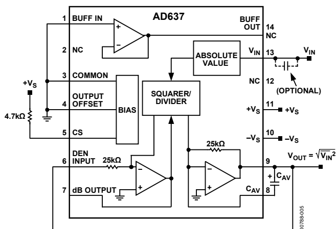
Figure 5. Standard RMS Connection
