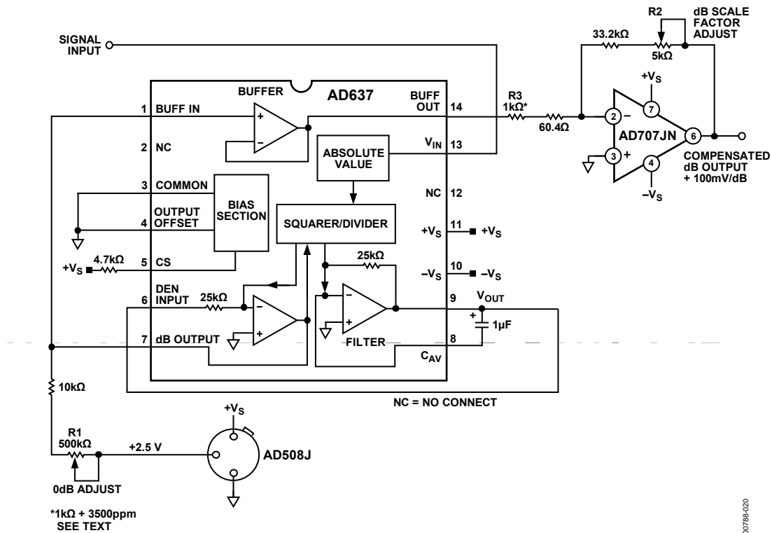
Figure 20. dB Connection
