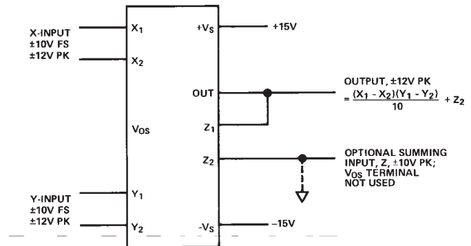
Figure 5. Basic Multiplier Connection
