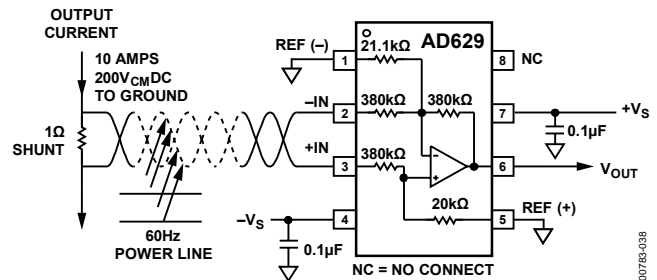
Figure 38. Error Budget Analysis Example 1: V_{IN} = 10 V Full-Scale, V_{CM} = 200 V DC, R_{SHUNT} = 1 \Omega , 1 V p-p, 60 Hz Power-Line Interference
