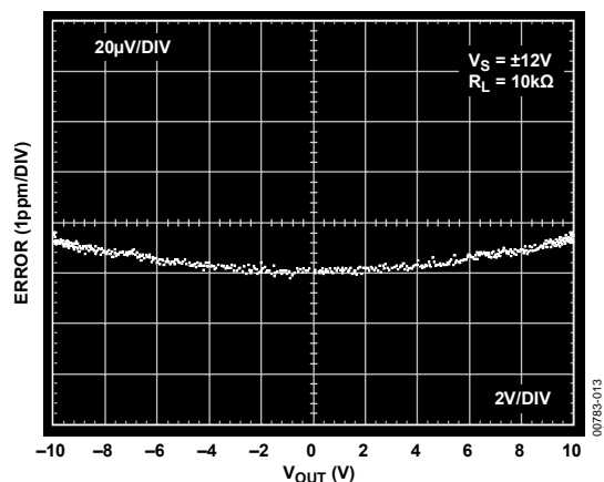
Figure 12. Gain Nonlinearity; V_S = \pm 12V , R_L = 10k\Omega
