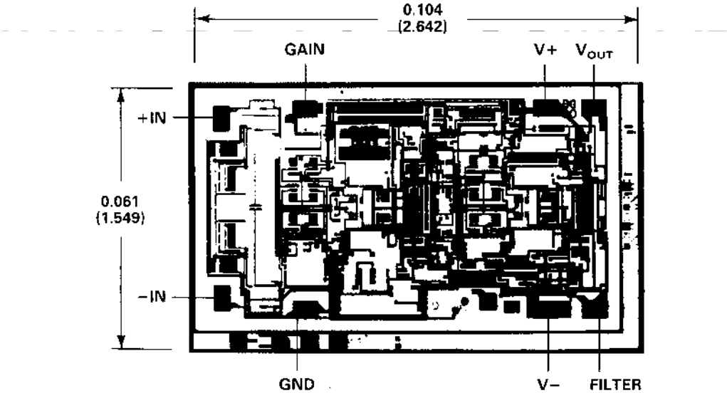
METALLIZATION PHOTOGRAPH Dimensions shown in inches and (mm).
