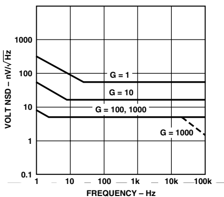
Figure 14. RTI Noise Spectral Density vs. Gain
