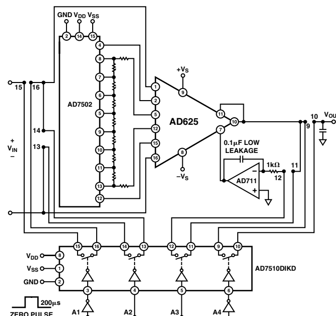
Figure 36. Auto-Zero Circuit
