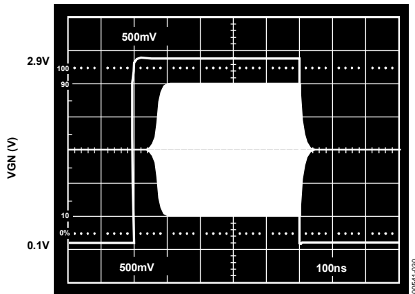
Figure 29. Gain Response
