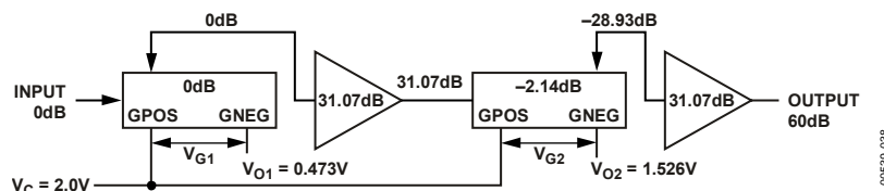
Figure 38. AD603 Gain Control Input Calculations for Sequential Control Operation V_C = 2.0 V
