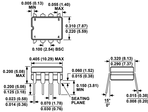
Figure 53. 8-Lead Ceramic Dual In-Line Package [CERDIP] (Q-8)
