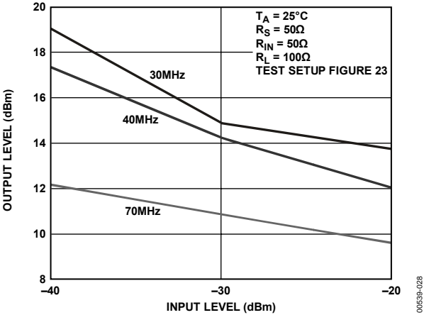
Figure 28. Third-Order Intercept -10 dB/+30 dB Mode, Gain = 30 dB
