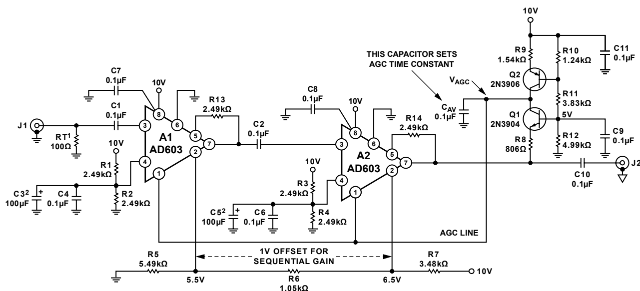
Figure 47. A Low Noise AGC Amplifier
