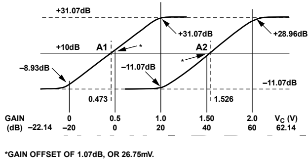
Figure 39. Explanation of Offset Calibration for Sequential Control
