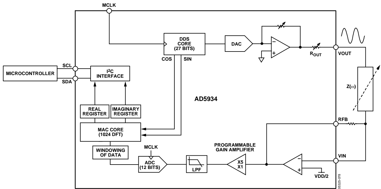
Figure 14. AD5934 Block Overview
